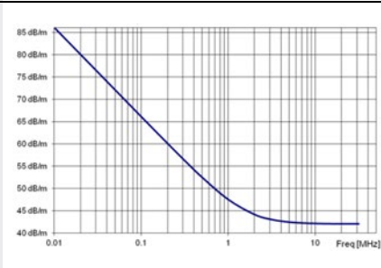
Antenna (Loop) 9 kHz to 30 MHz
