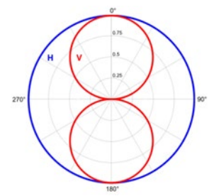
Antenna (Loop) 9 kHz to 30 MHz
